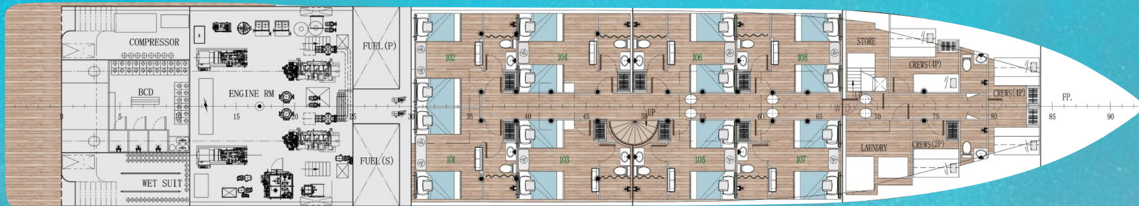
LOWER DECK
